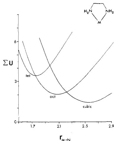
Figure 15. Strain energy, \Sigma U , of an isolated five-membered chelate ring involving ethylenediamine, calculated using molecular mechanics, as a function of metal-nitrogen bond length and N-M-N bond angles appropriate to different coordination geometries. 69 The N-M-N angles used were 109.5^\circ for tetrahedral, 90^\circ for octahedral (or square planar), and 70^\circ for cubic. As metal ions become larger, coordination numbers increase, and so preferred N-M-N angle decreases. The diagram shows that the lowest strain energy for the ethylenediamine type of chelate ring is achieved with metal ions with longer M-N bond lengths (and smaller N-M-N angles), i.e., large metal ions.
