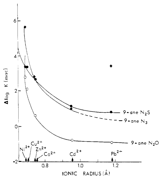
Figure 22. Size-match selectivity of 9-aneX 3 type macrocycles. The change in formation constant, \Delta \log K_1 , produced by adding an ethylene bridge to an open-chain \text{NH}_2\text{CH}_2\text{CH}_2\text{XCH}_2\text{CH}_2\text{NH}_2 ligand to produce a 9-aneN 2 X macrocycle, where X = S (●), O (○), or NH (◆), is plotted against metal ionic radius. After ref 78. The values of \Delta \log K_1 are a maximum for metal ions of the size of high-spin Ni(II), which molecular mechanics calculations 78 show to be the optimum size for coordinating to 9-aneN 2 X type macrocycles. Data from ref 21 and 78, ionic strength 0.1 M, 25 °C.
