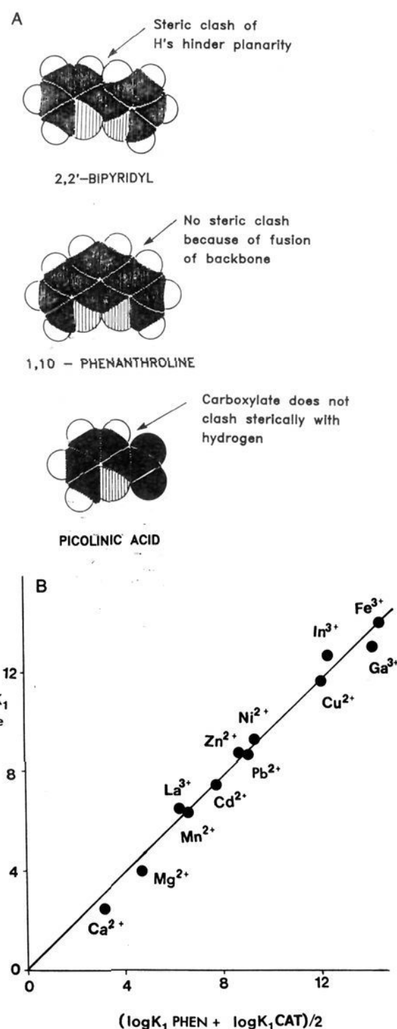
Figure 11. (A) Steric clash in 2,2-bipyridyl which hinders planarity and lowers complex stability relative to 1,10-phenanthroline and picolinic acid, where the clash is not present. (B) The rule of average environment in complex stability, as exemplified by the relationship between \log K_1 for the 8-hydroxyquinoline (oxine) complex and the average of \log K_1 for the 1,10-phenanthroline (PHEN) complex + \log K_1 for the catechol (CAT) complex. Data from ref 21, ionic strength 0.1 M, 25 °C.
