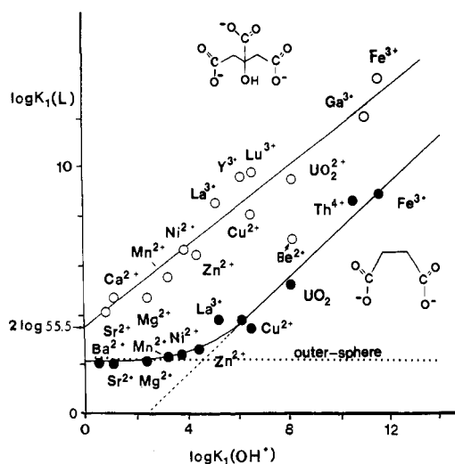
Figure 6. Relationship between the formation constants for citrate (O) and for succinate (●) and \log K_1(\text{OH}^+) for a variety of metal ions. The relationship for citrate shows the intercept of 2 \log 55.5 as expected 30,31 for tridentate ligands, but the \text{Be}^{2+} ion shows a drop in complex stability because of steric difficulties in coordinating all three donor atoms. The relationship for succinate shows a negative intercept because of the entropy associated with immobilizing the long bridge between the donor groups. The dotted line is the calculated 32 stability for the outer-sphere complexes between dipositive cations and dinegative anions. Data from ref 21, ionic strength, 0, 25 °C.
