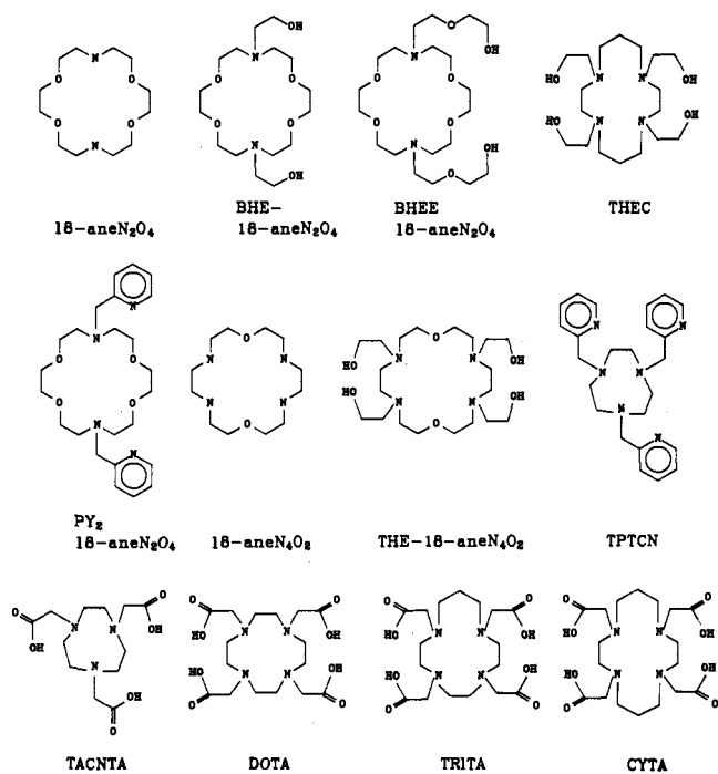
Figure 27. Structures of some ligands discussed in this review.
