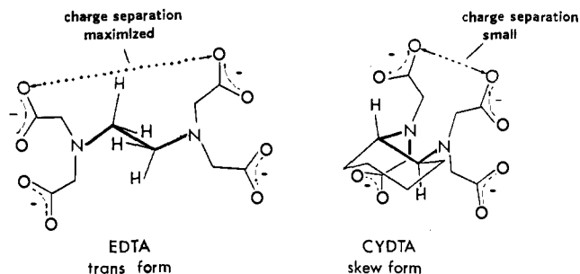
Figure 36. Role of preorganization in the complex stability of EDTA type ligands. In EDTA it appears 143 that the free ligand in solution adopts the trans form so as to maximize charge separation, whereas CYDTA is preorganized into the skew form for complex formation, which leads to increases in complex stability. 21
