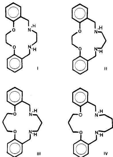
Figure 23. Some ligands studied by Lindoy et al. 84-98
